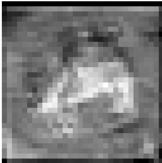
Feature Map 2
