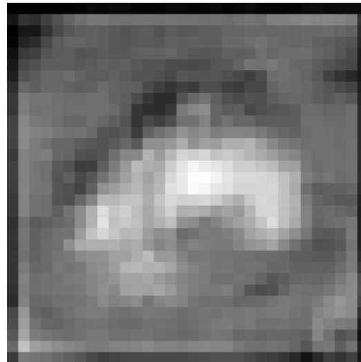
Feature Map 4
