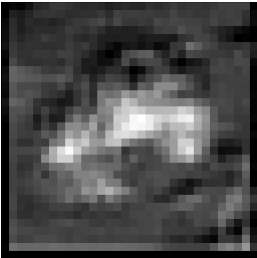
Feature Map 1
