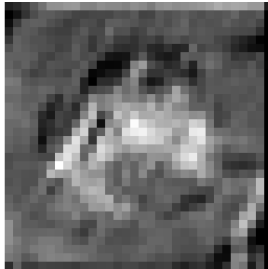
Feature Map 3
