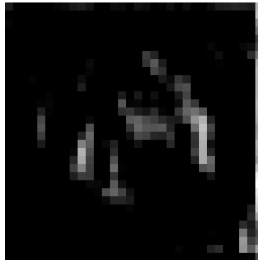
Feature Map 8
