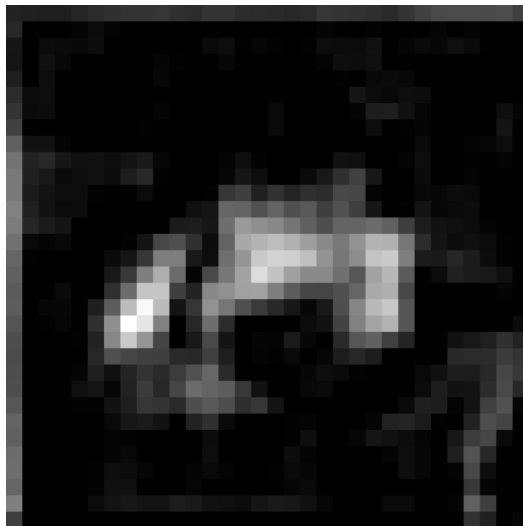
Feature Map 6
