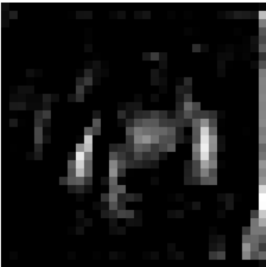
Feature Map 5
